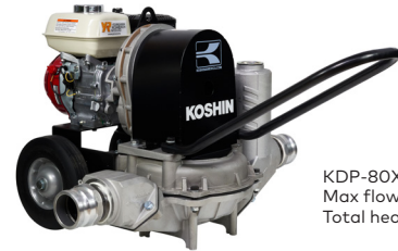
KDP-50X 2" (50mm) Max flow 197 L/min Total head 7.6m
